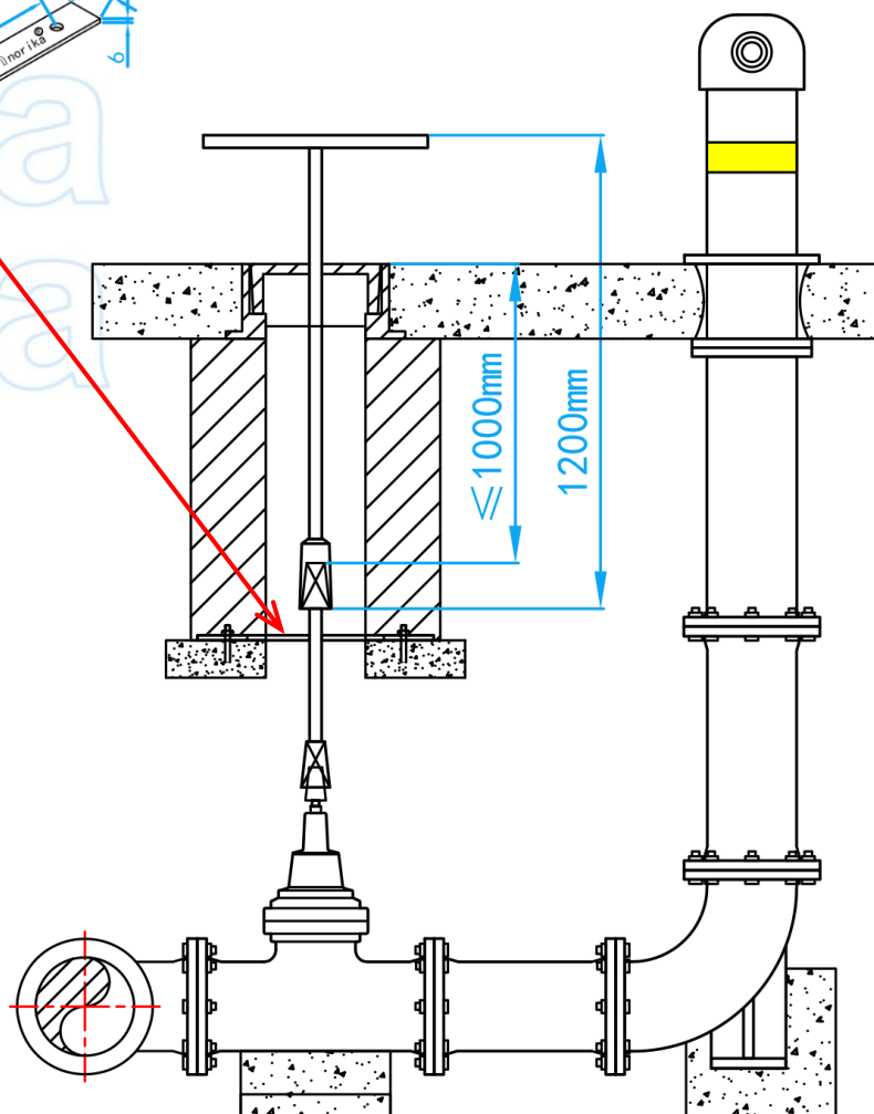
INSTALLATION ASSEMBLY
